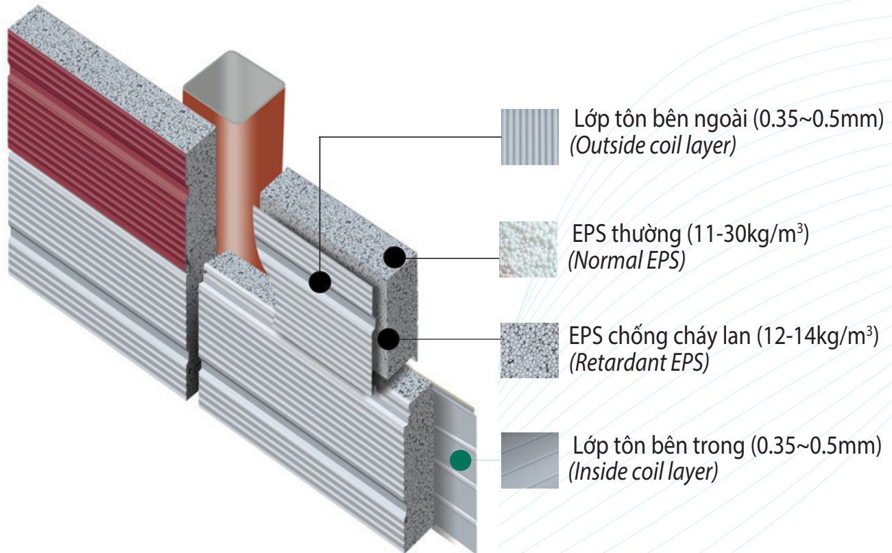
Cấu tạo tấm Sandwich Panel Korea/ Korea Sandwich Panel detail
