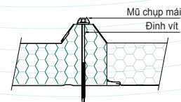
Mỗi nối 2 tấm/Joint detail
